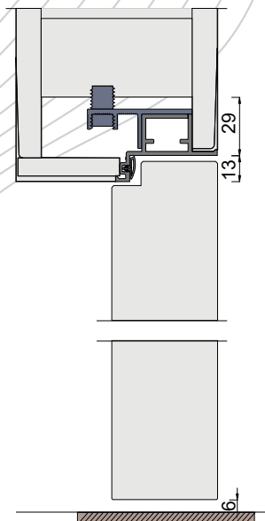
outward opening
